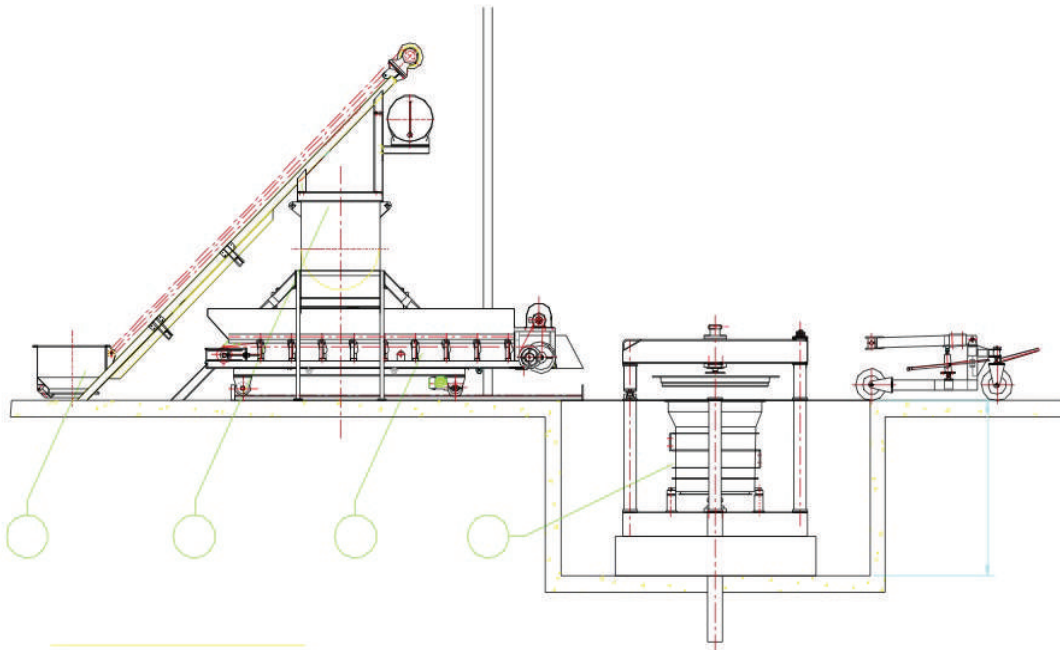
Typical bucket sledge conveyor, concrete mixer and feeding belt pipe machine layout
